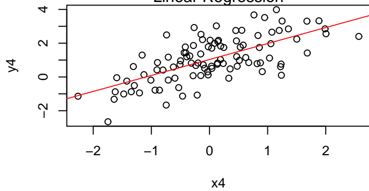
y4 vs. x4 Linear Regression
