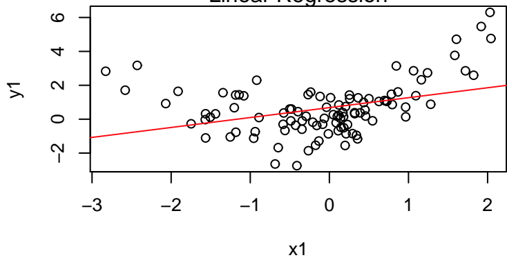
y1 vs. x1 Linear Regression
