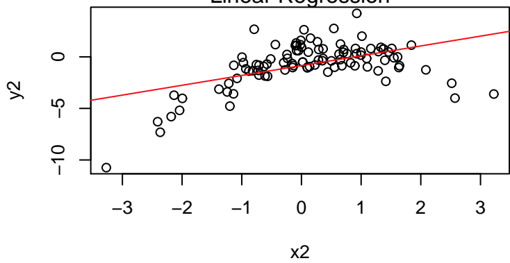
y2 vs. x2 Linear Regression
