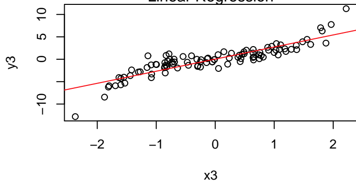
y3 vs. x3 Linear Regression
