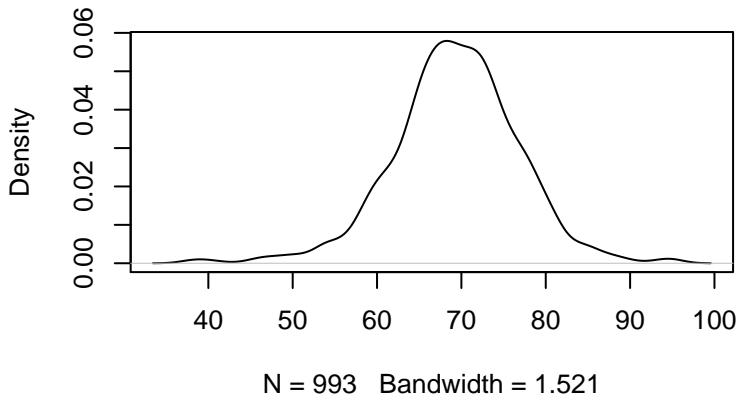
Kernel Density Plot of Actuals
