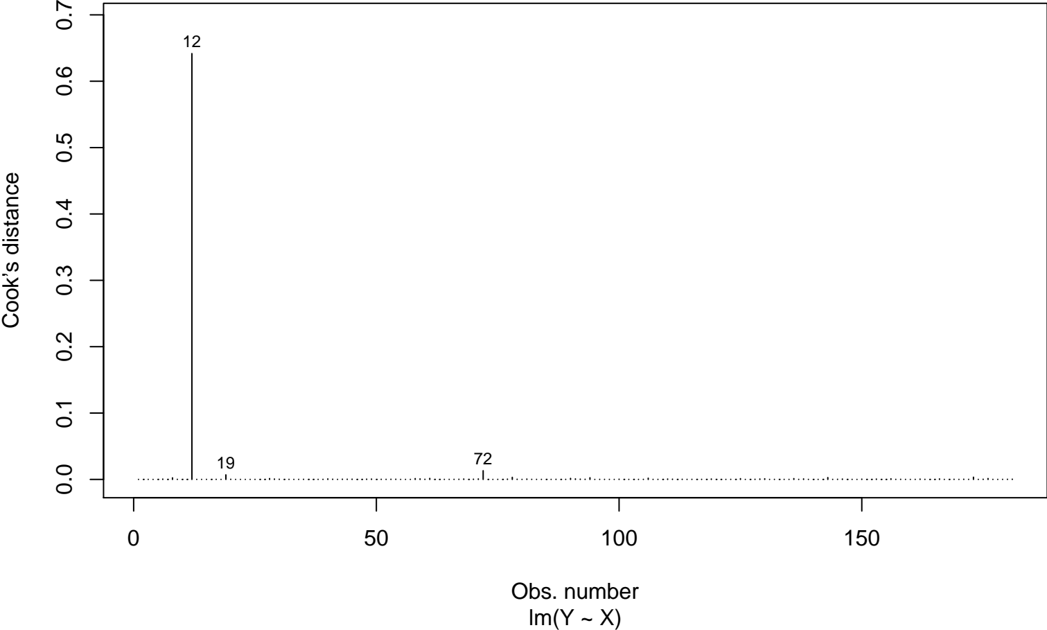
Cook's distance
