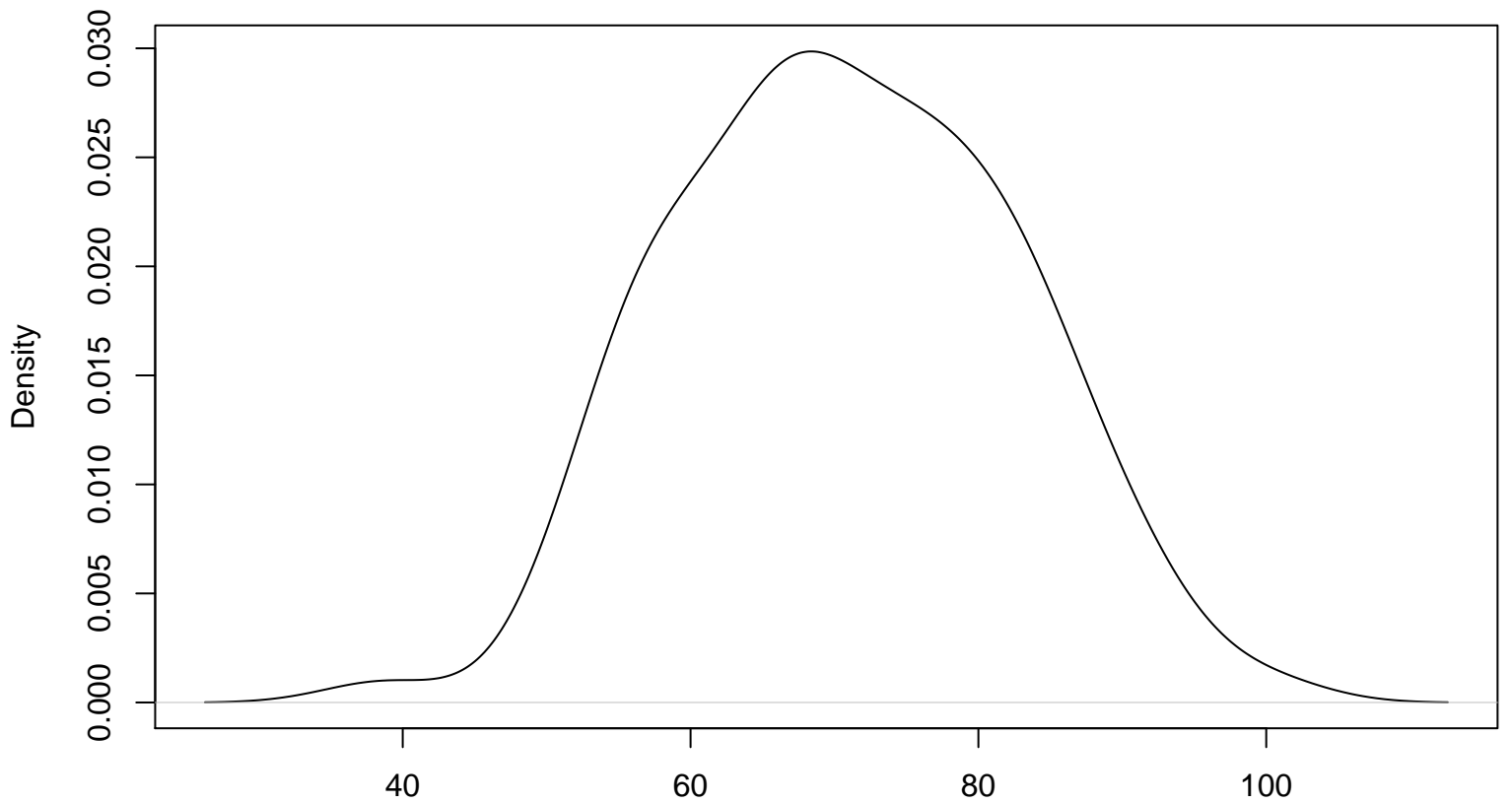
Kernel Density Plot of Sample 1
