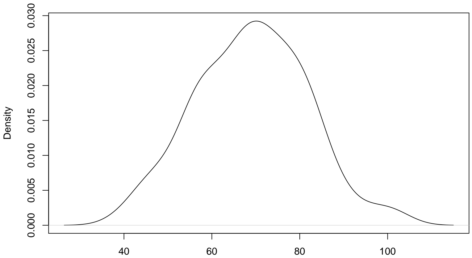
Kernel Density Plot of Sample 3
