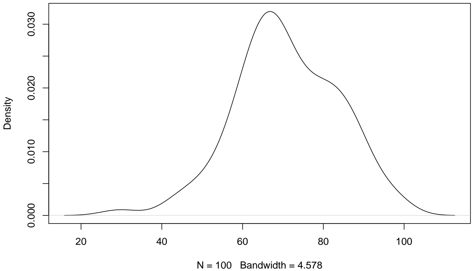
Kernel Density Plot of Sample 1
