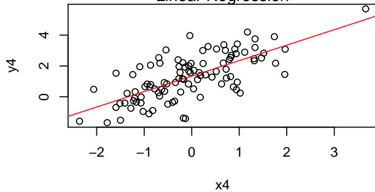
y4 vs. x4 Linear Regression
