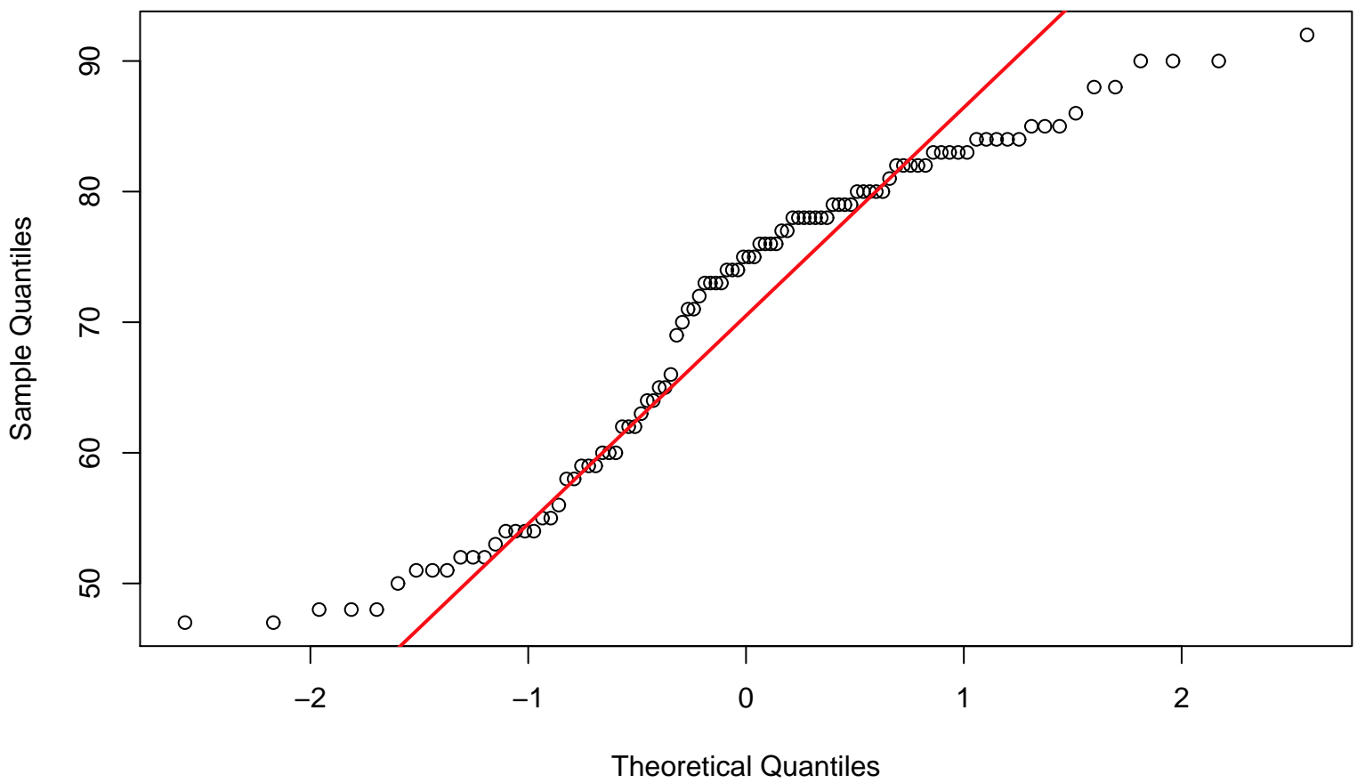
Normal Q-Q Plot Sample 2
