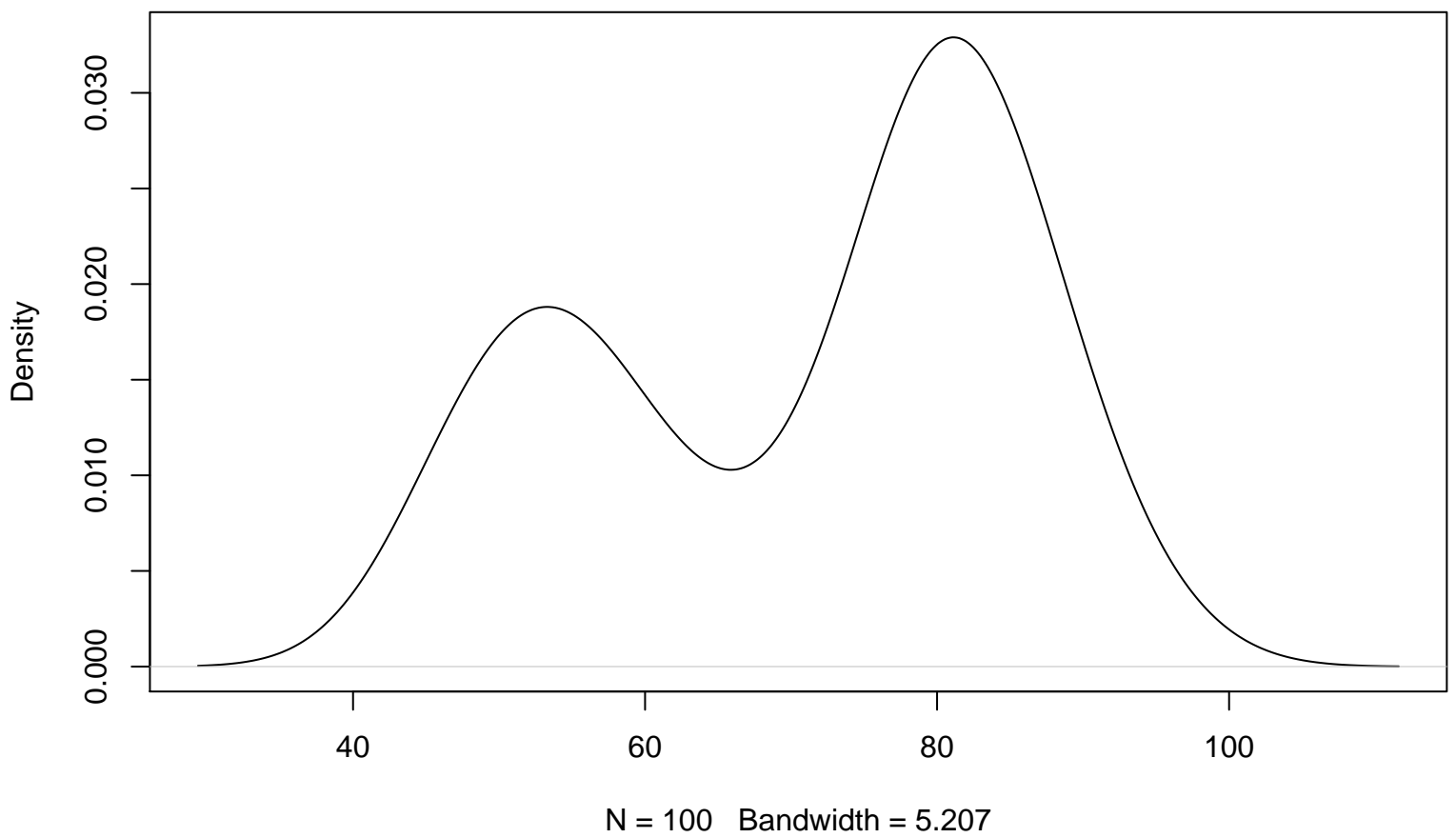
Kernel Density Plot of Sample 3
