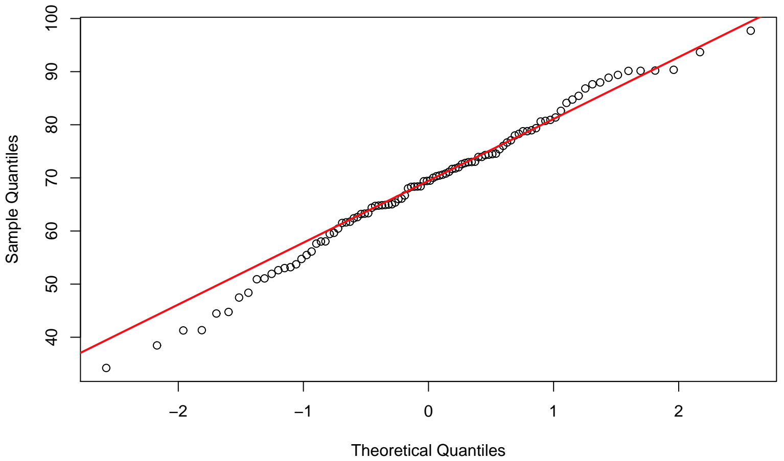
Normal Q-Q Plot Sample 2
