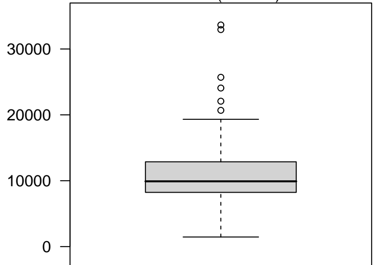
Node 3 (n = 225)
