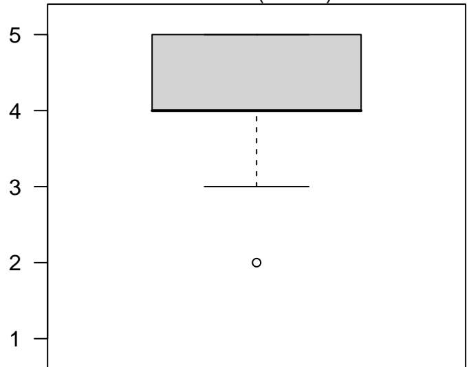
Node 3 (n = 25)
