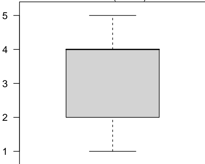
Node 2 (n = 32)
