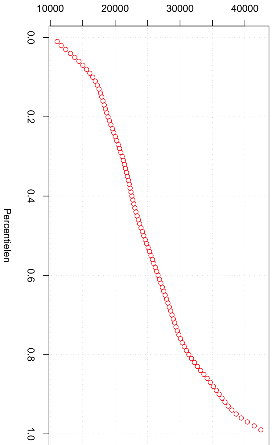
Harrell-Davis Quantiles
