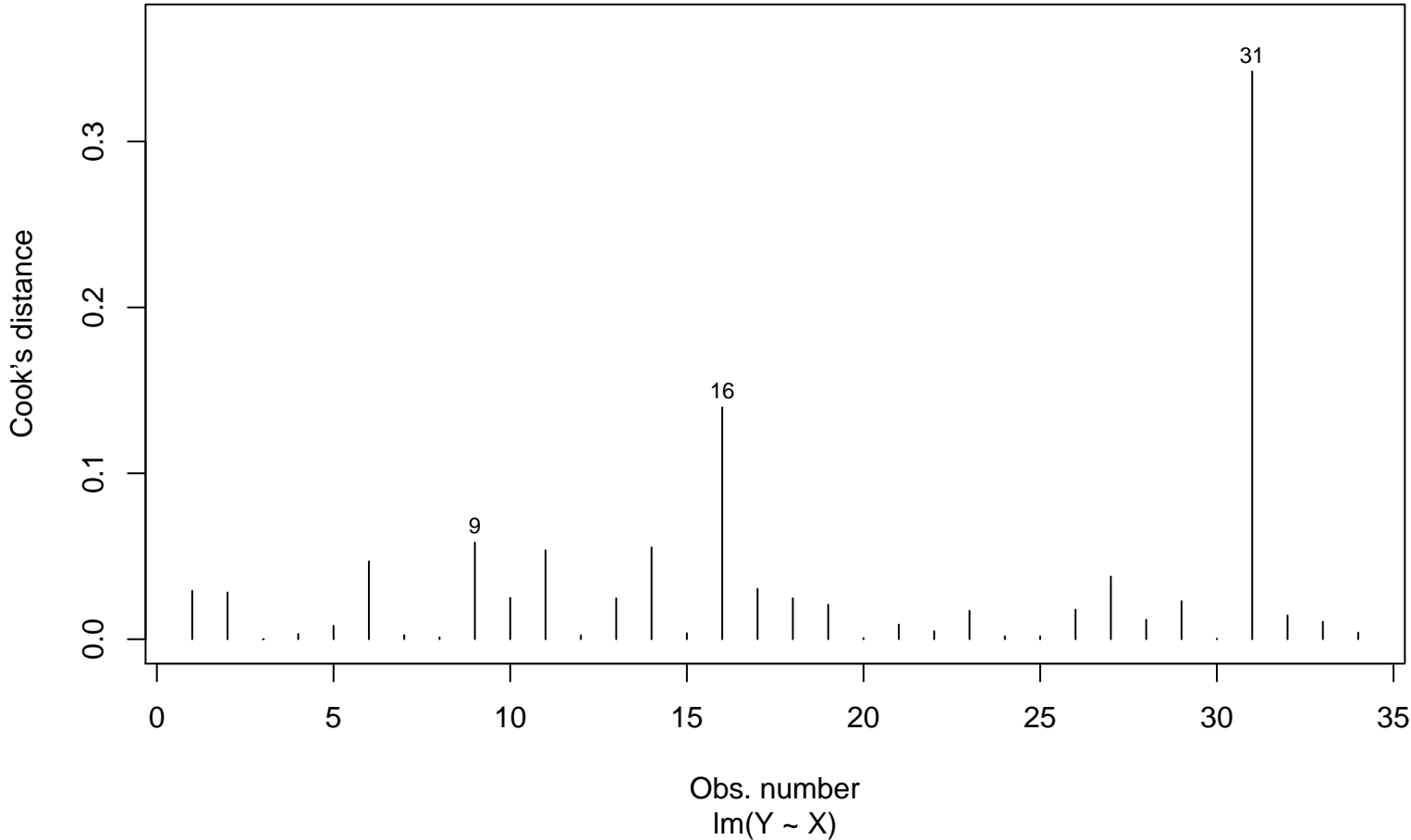
Cook's distance
