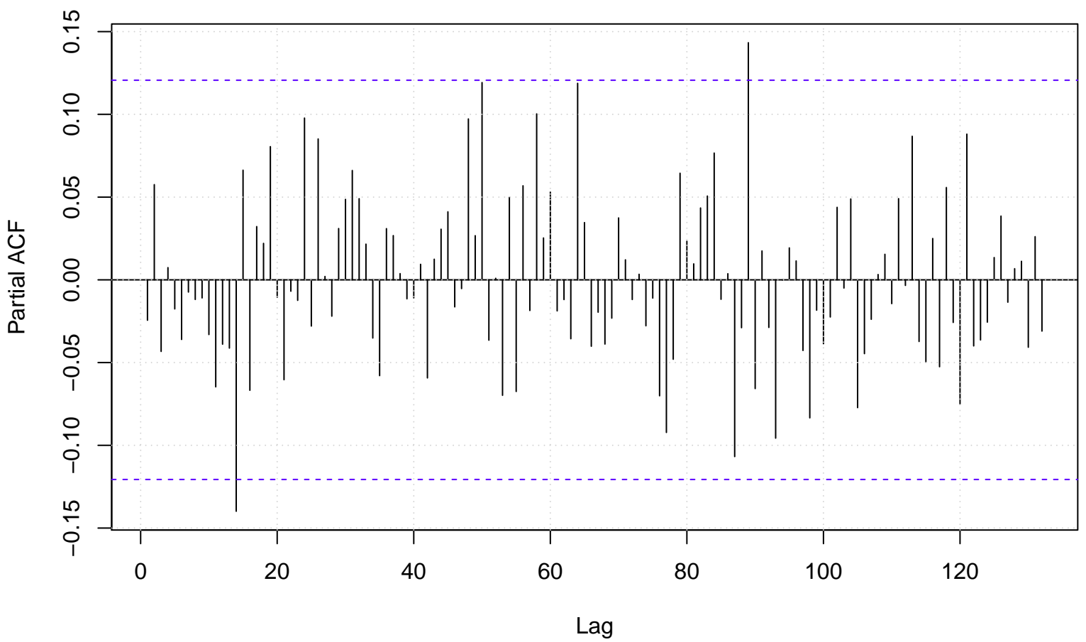
Residual Partial Autocorrelation Function
