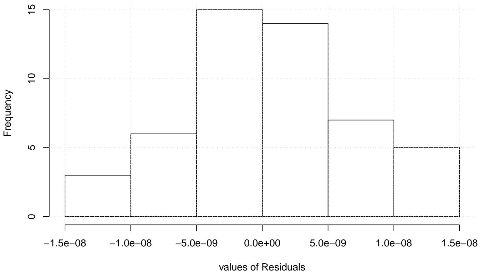
Residual Histogram
