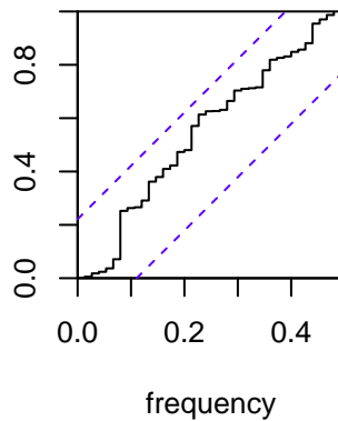
Standardized Residuals
