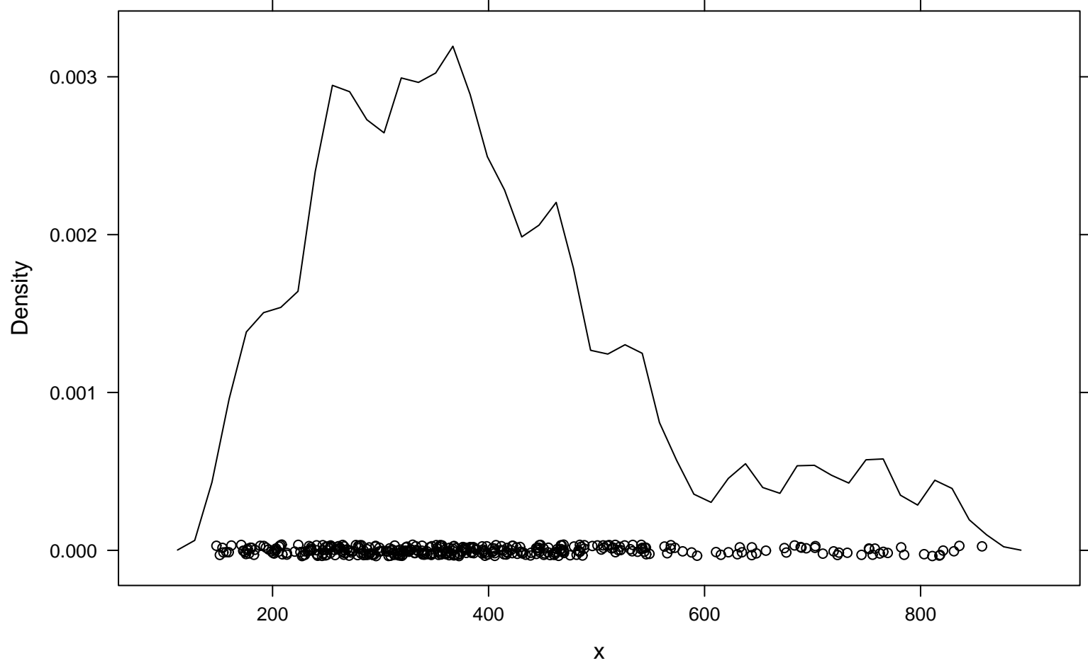
Density Plot bw = 12
