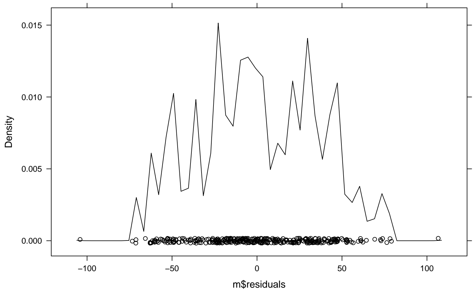
Density Plot bw = 0.65
