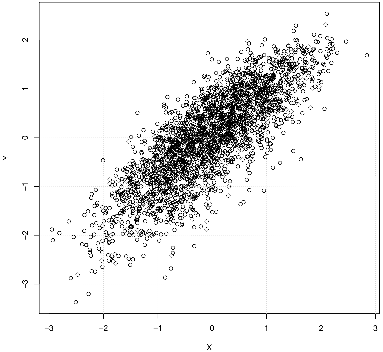
Scatterplot
