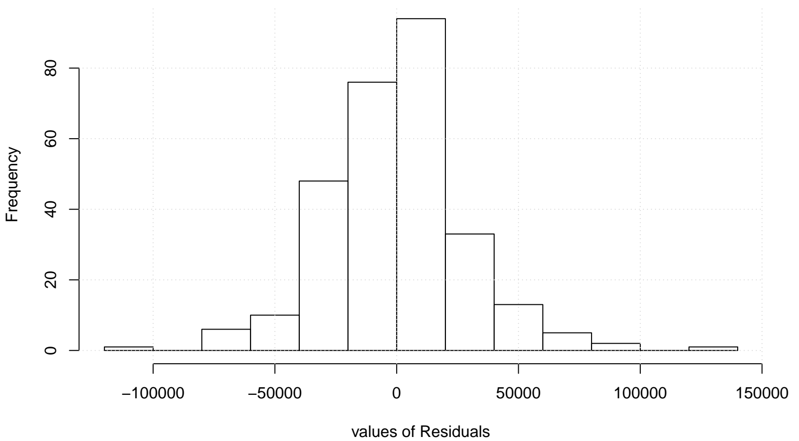
Residual Histogram
