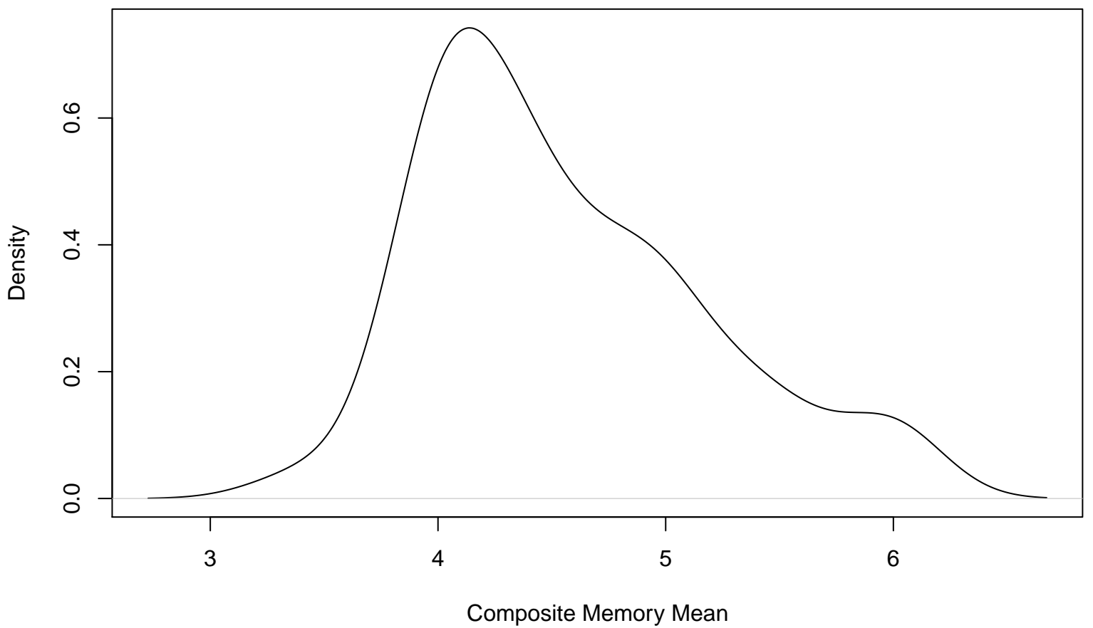
WW7 Compmemo Mean Distributional Plot
