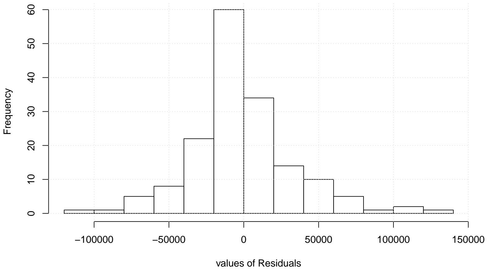
Residual Histogram
