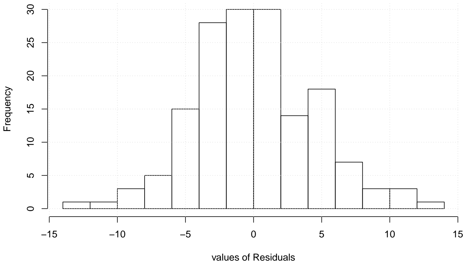
Residual Histogram
