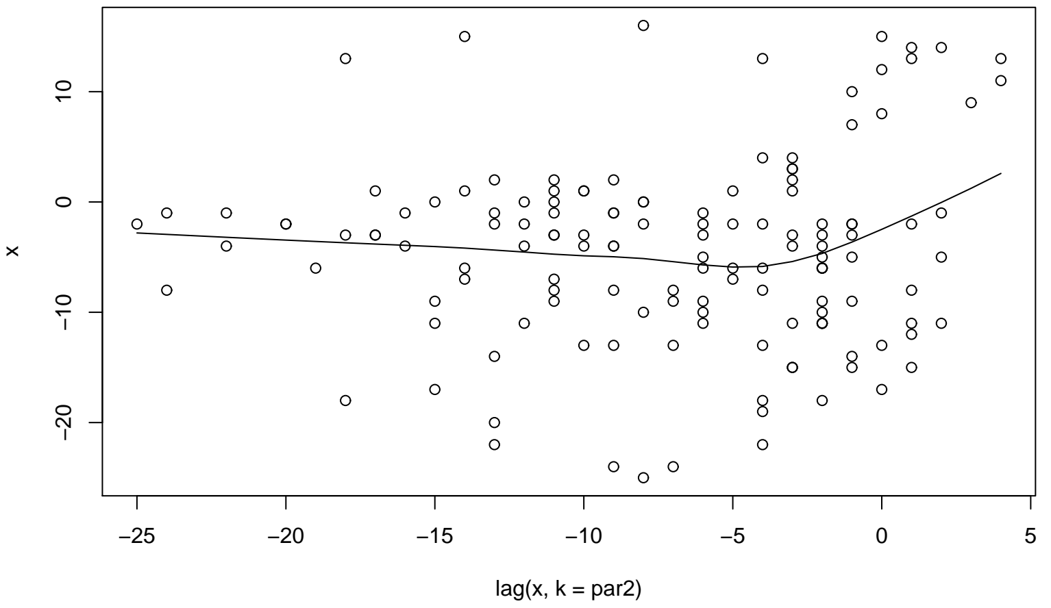
Lag plot (k=16), and lowess
