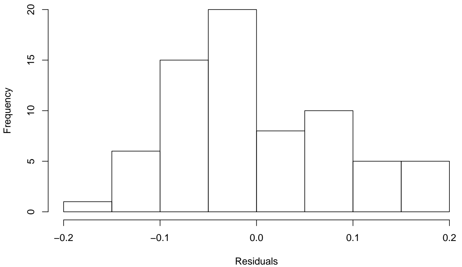
Residual Histogram
