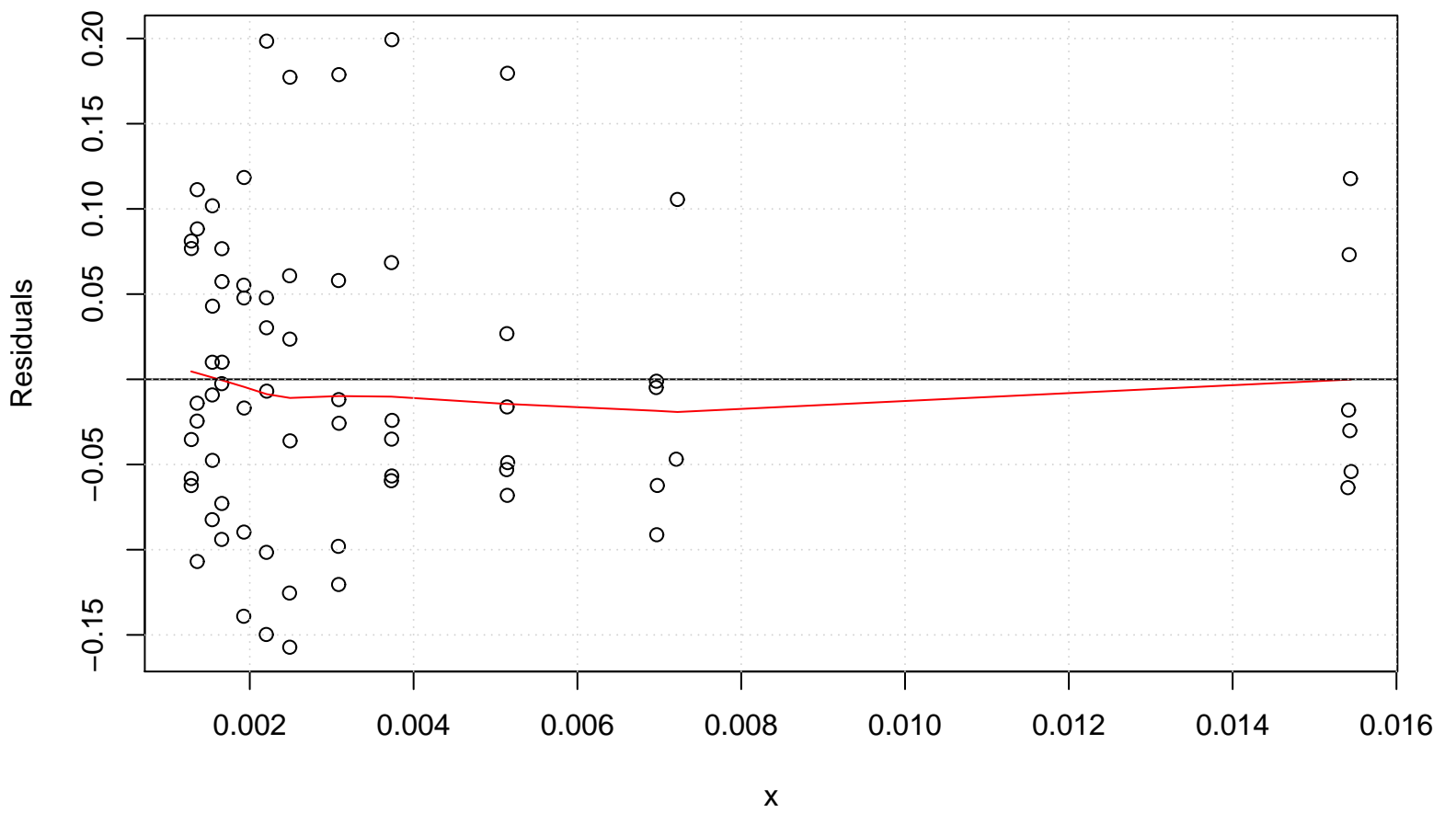
Scatterplot, lowess, and regression line
