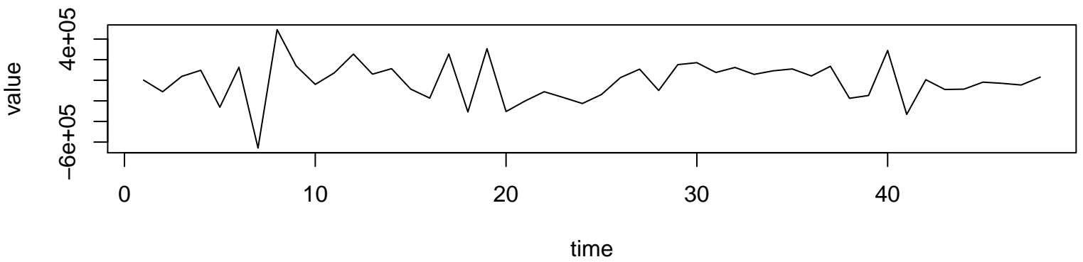
Working Time Series (lambda=1, d=0, D=2)
