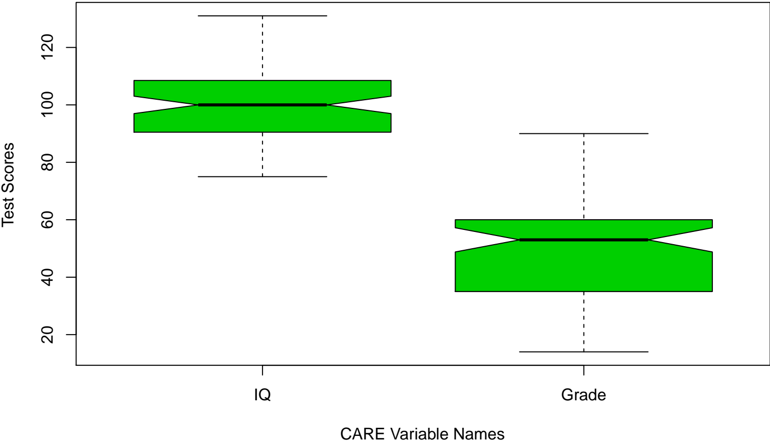
Relationship – average grade and IQ score
