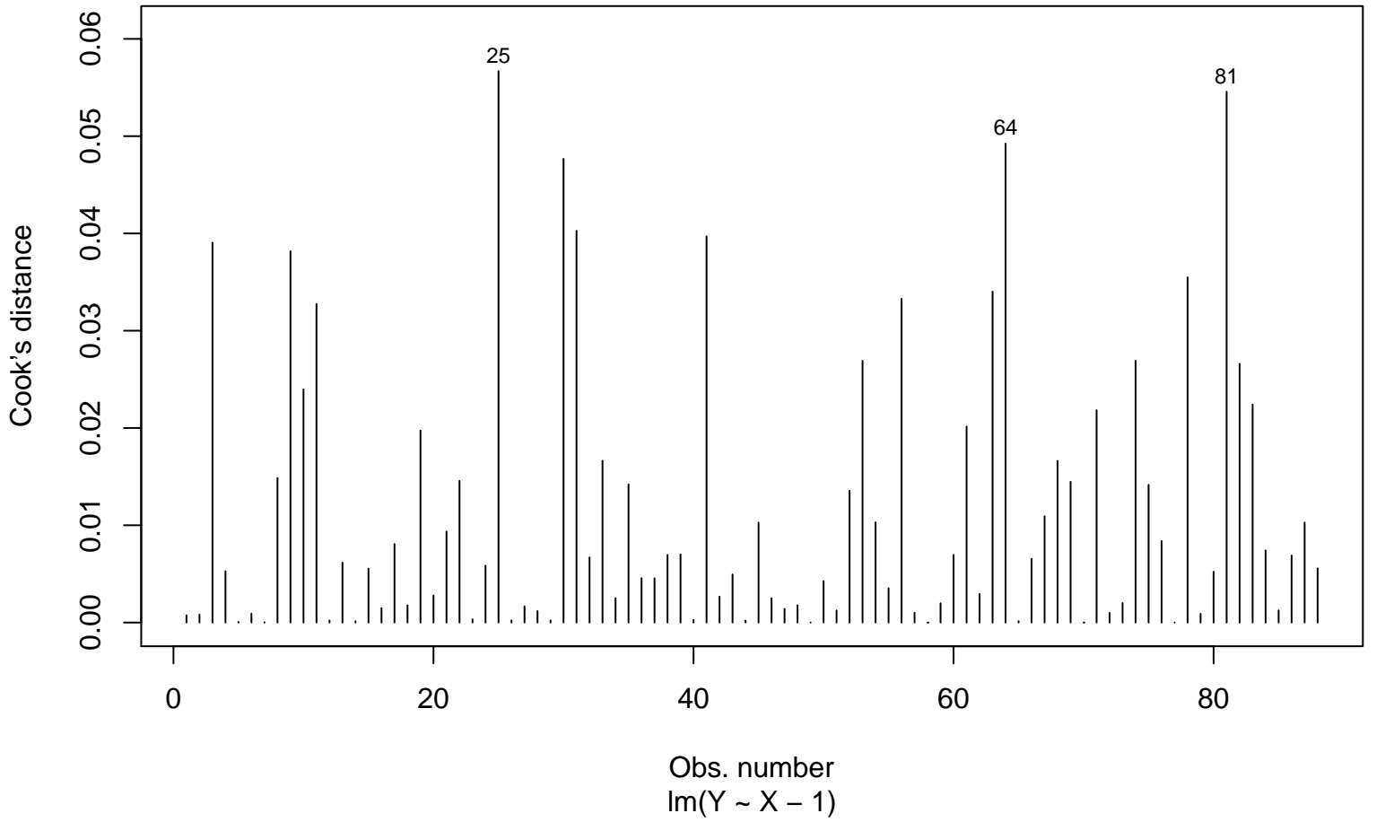
Cook's distance
