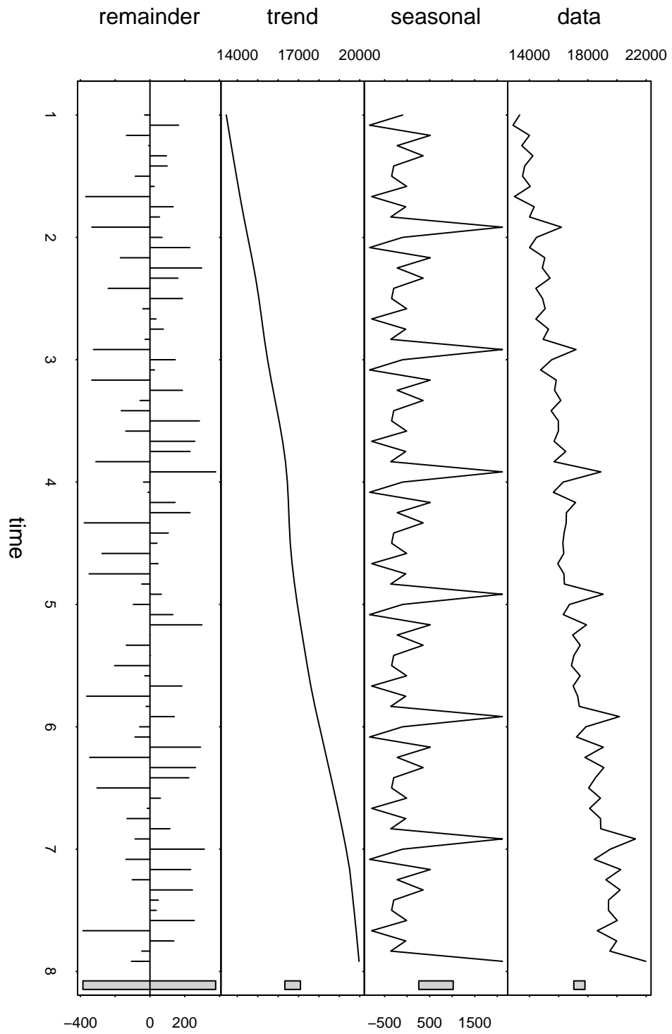
Seasonal Decomposition by Loess
