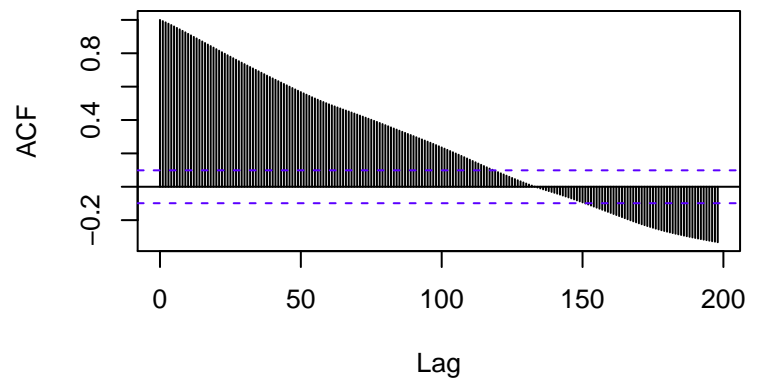
Random
