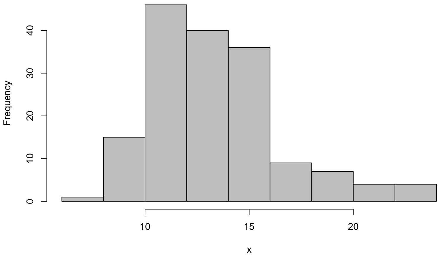
Histogram: Depression
