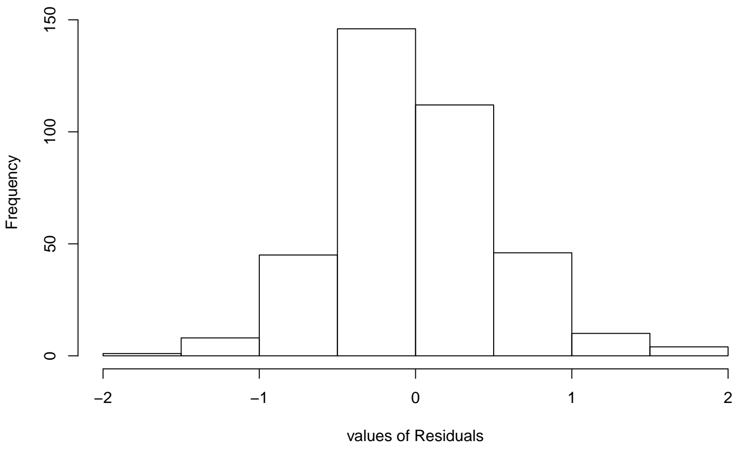
Residual Histogram
