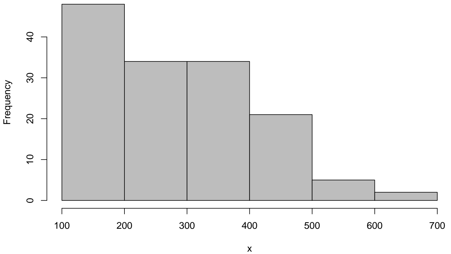
Histogram 2
