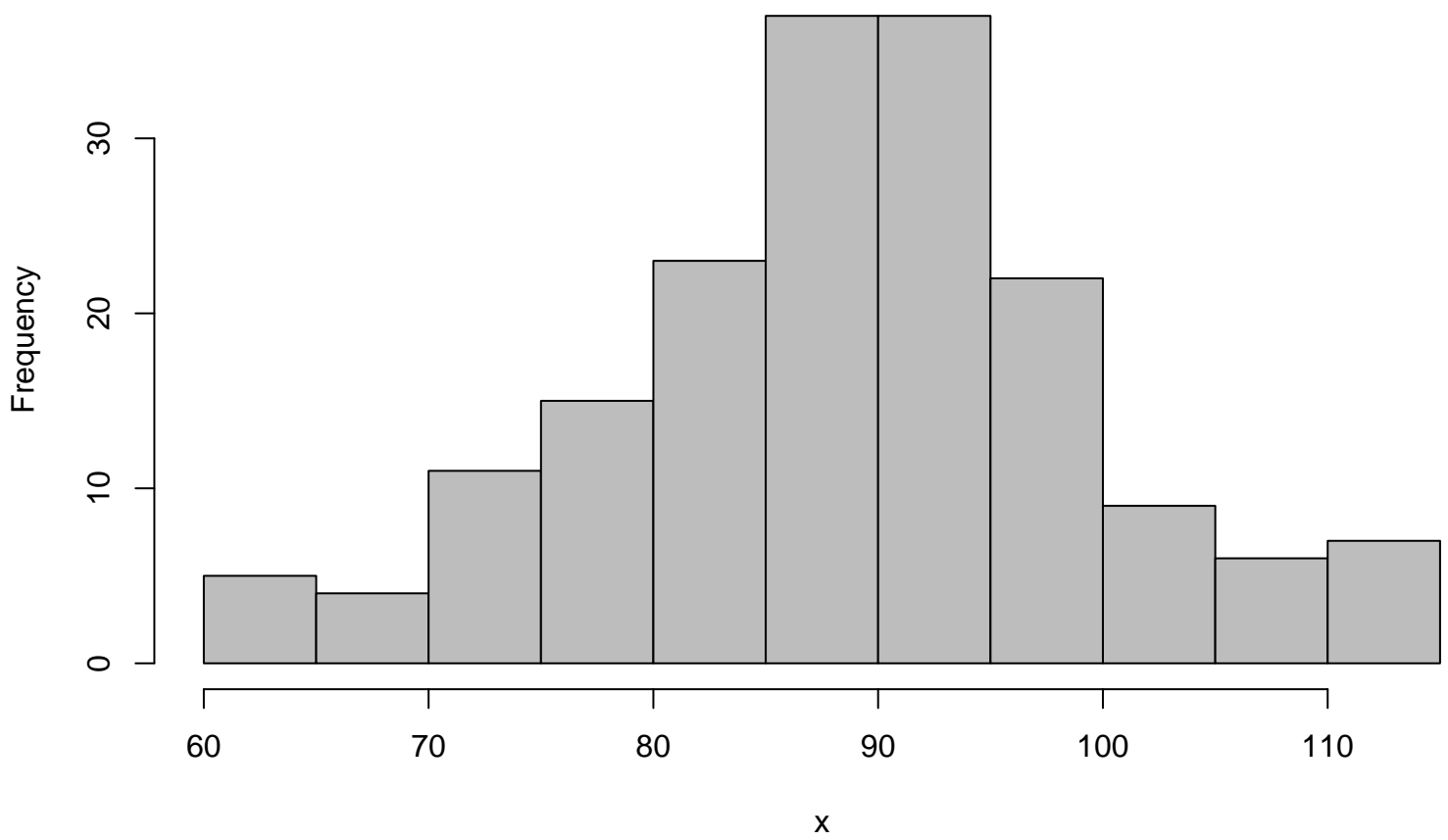
EG Histogram of WS1 data
