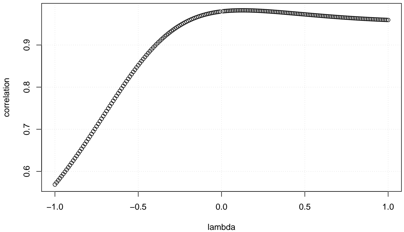
PPCC Plot – Tukey lambda
