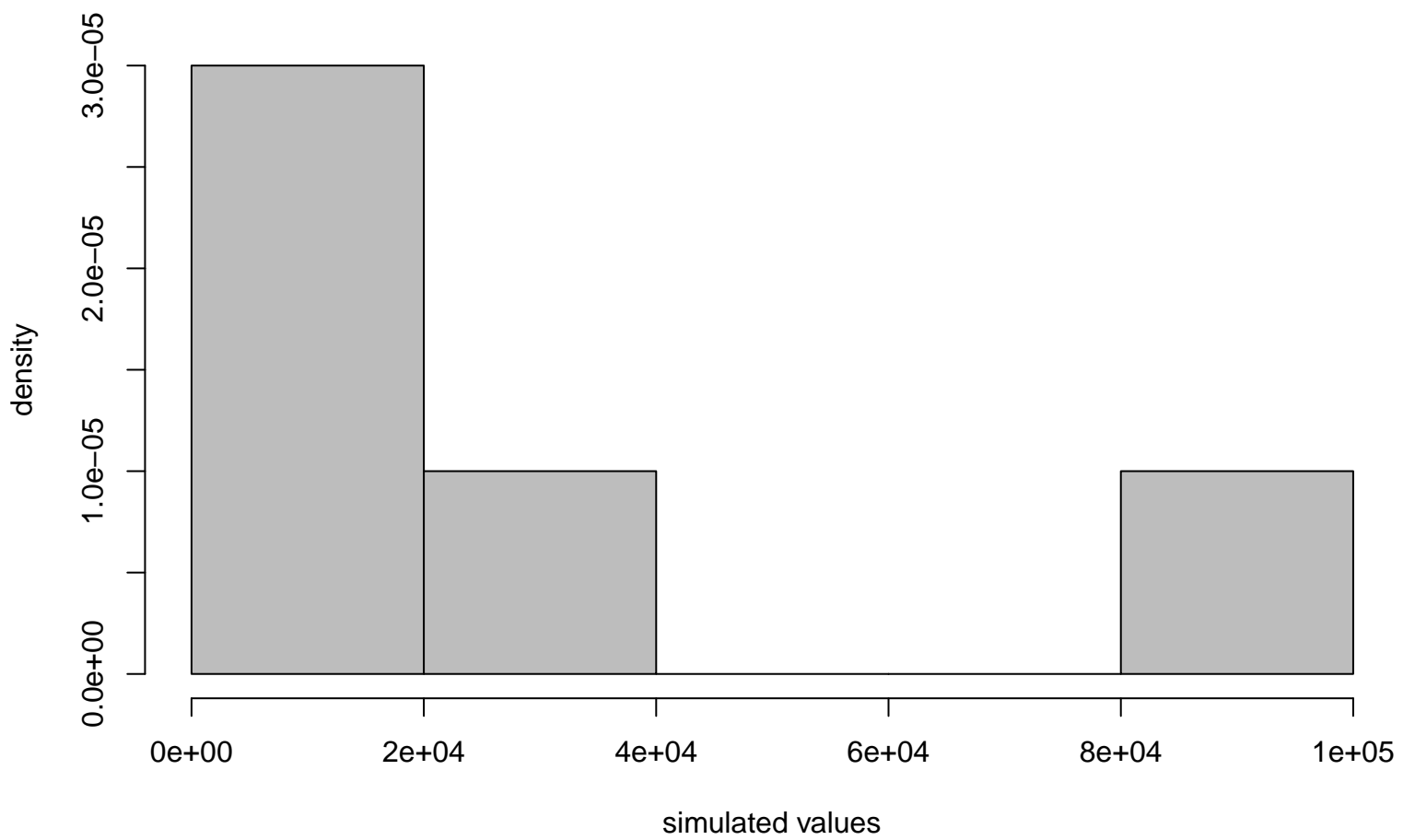
Histogram of 1st simulated series
