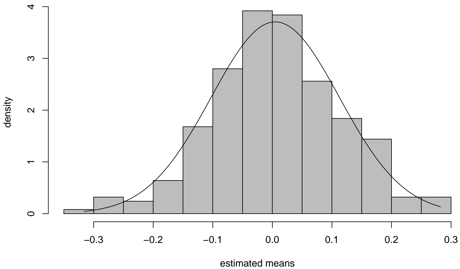
Histogram of Estimated Means
