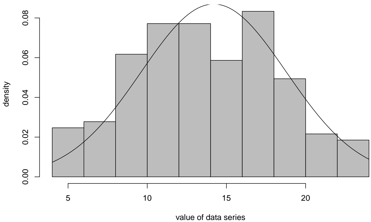
Histogram and Fitted Normal Density I3
