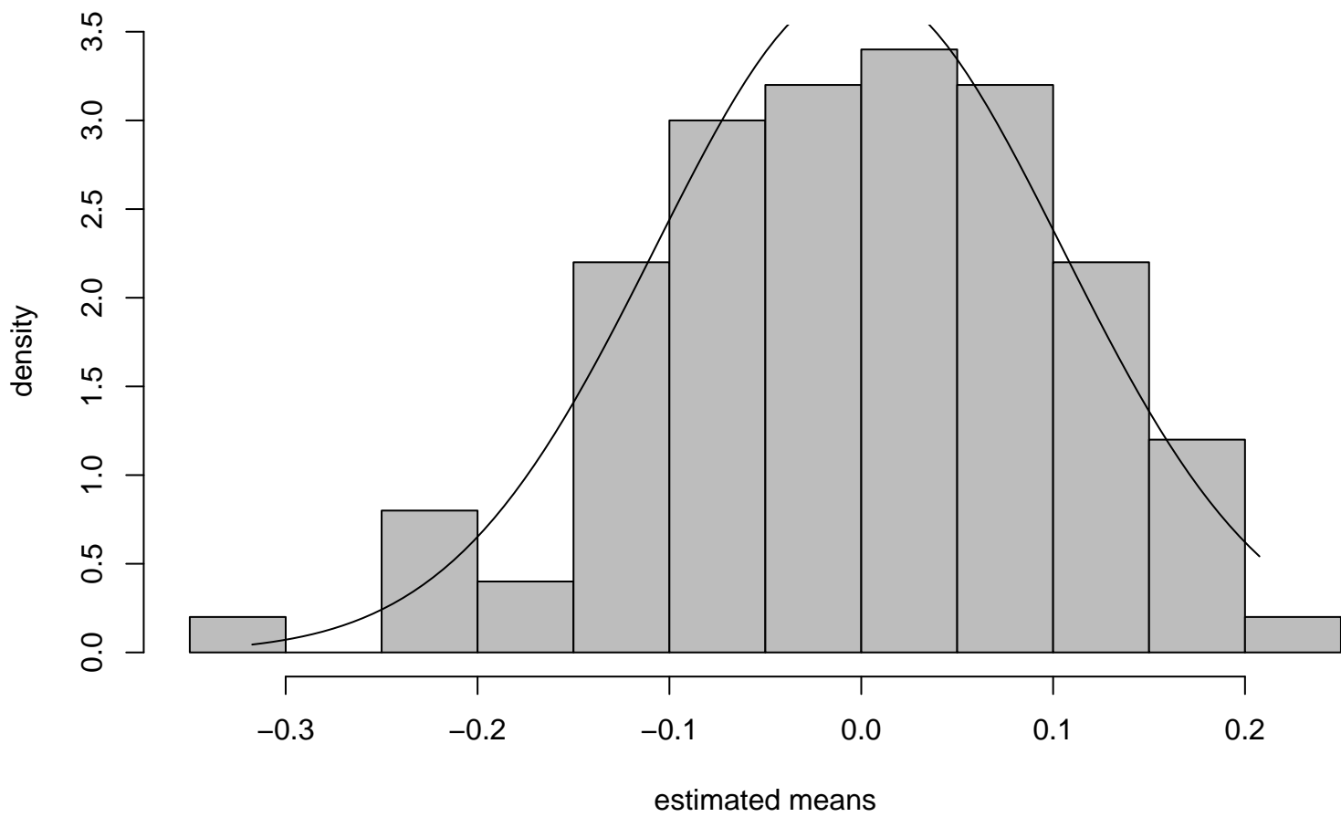
Histogram of Estimated Means
