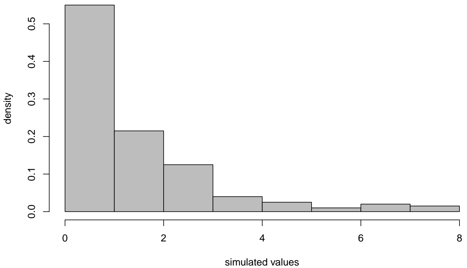
Histogram of 1st simulated series
