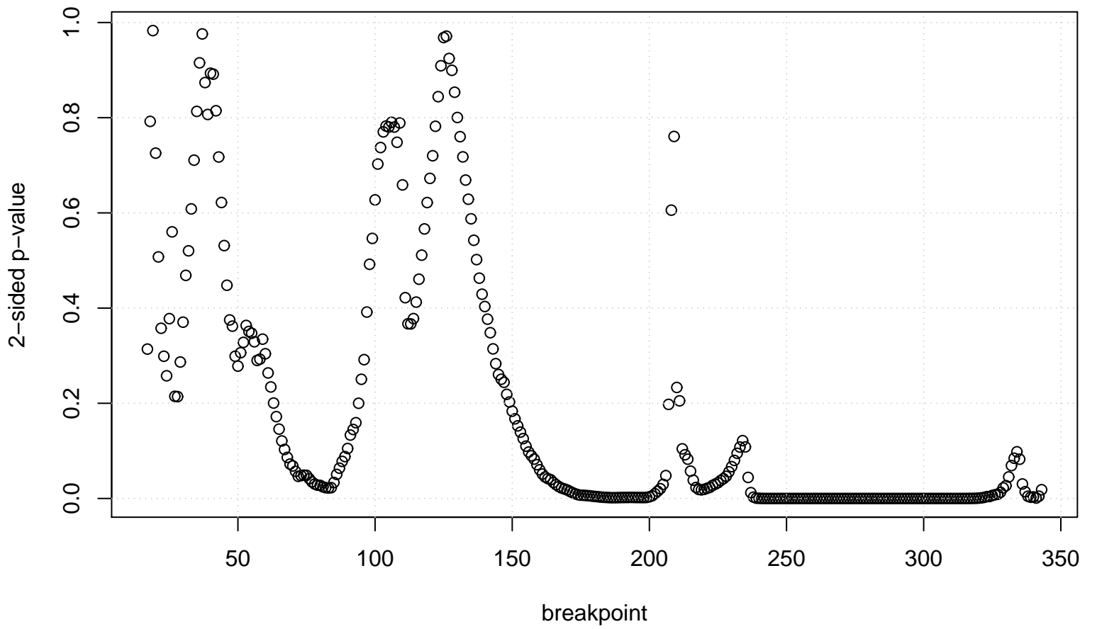
Goldfeld-Quandt test
