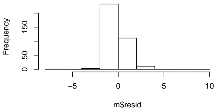
Residual Histogram
