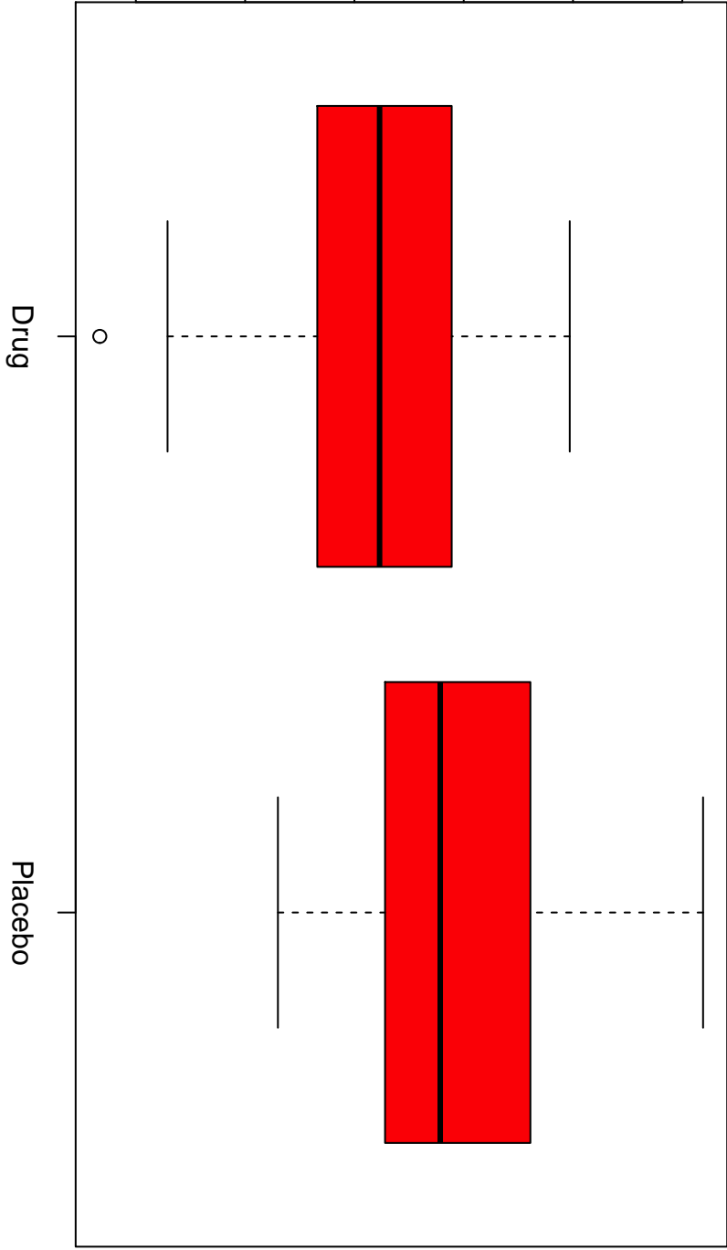
Boxplots Title
