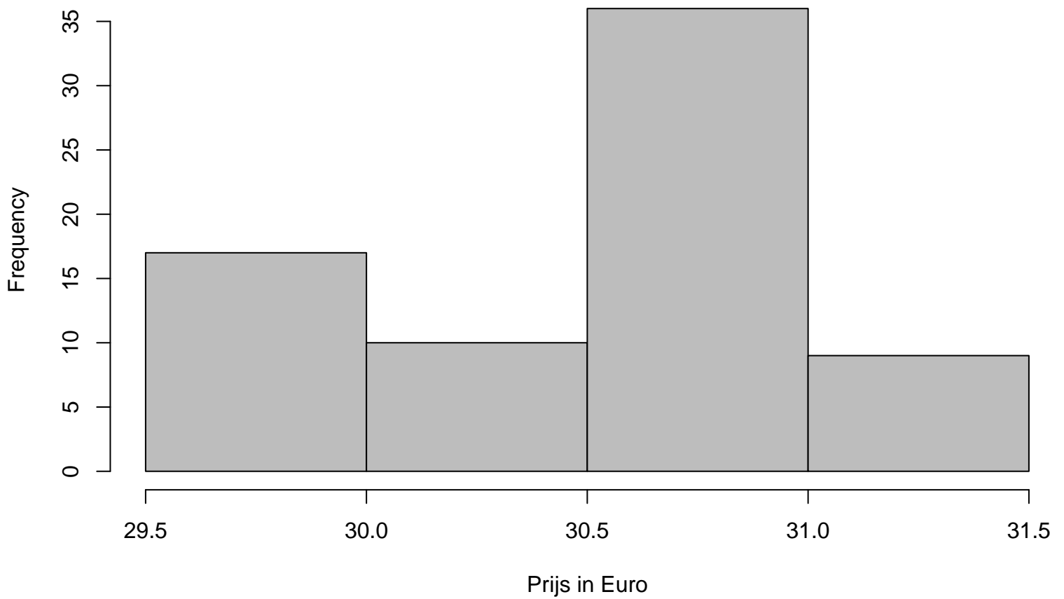
Histogram (5)
