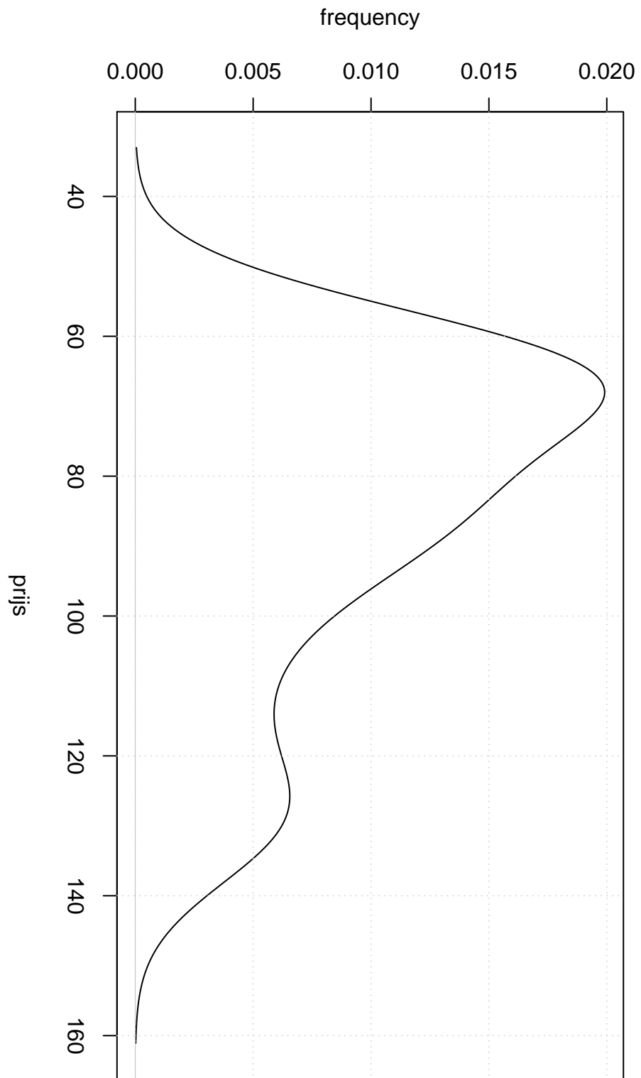
Gaussian Kernel
