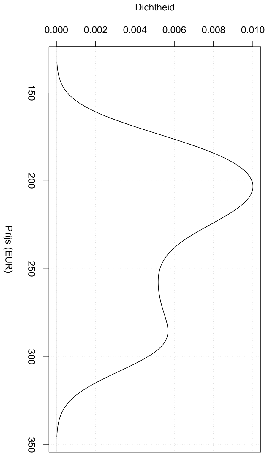
Gaussian Kernel
