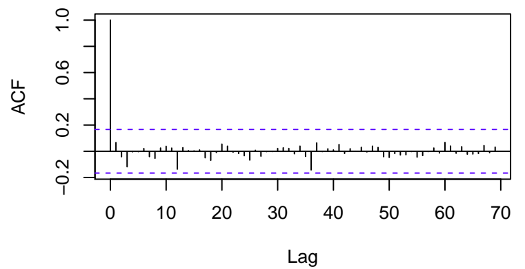
Standardized Residuals
