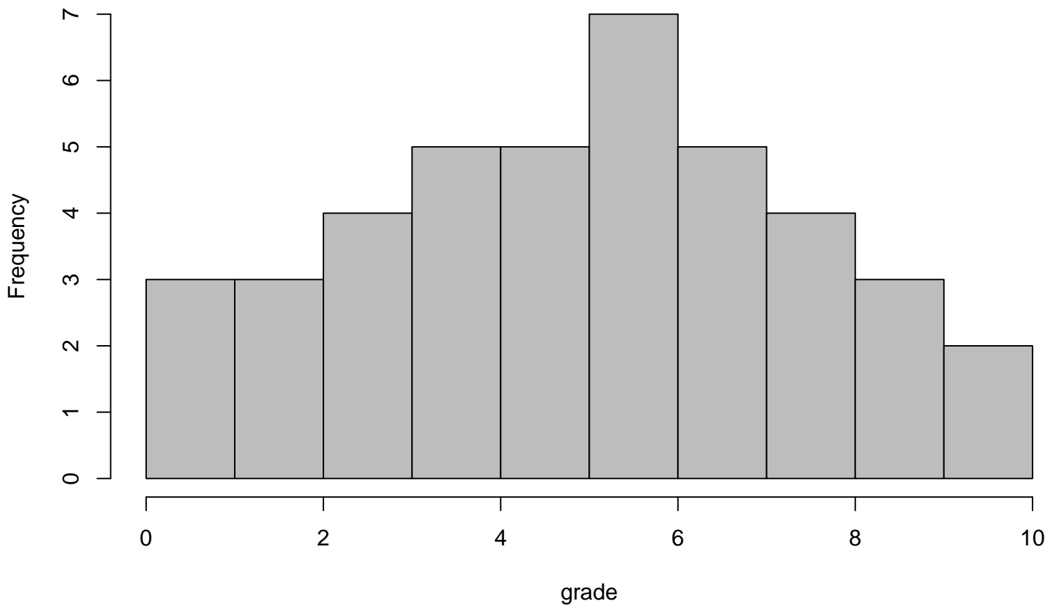
Histogram
